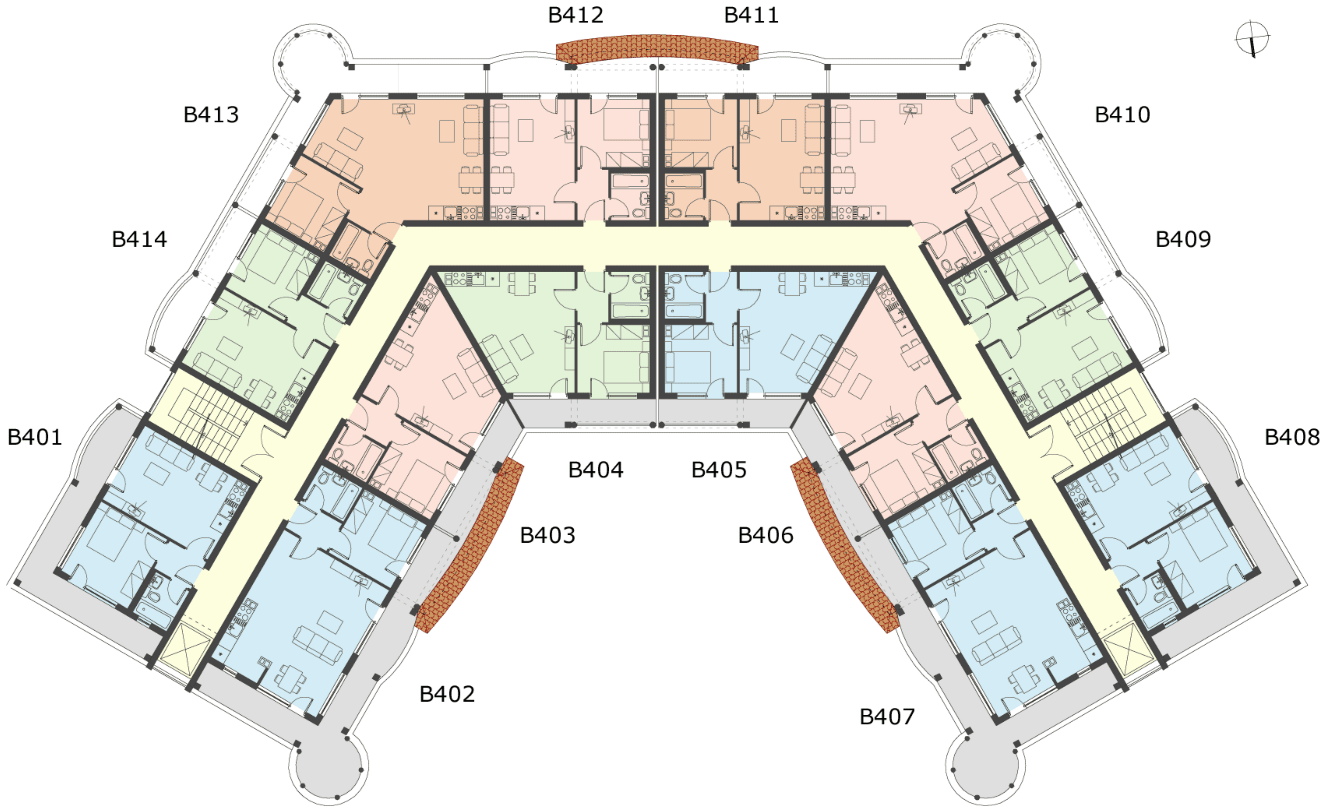
Block BI, floor 4 (+8.40)
