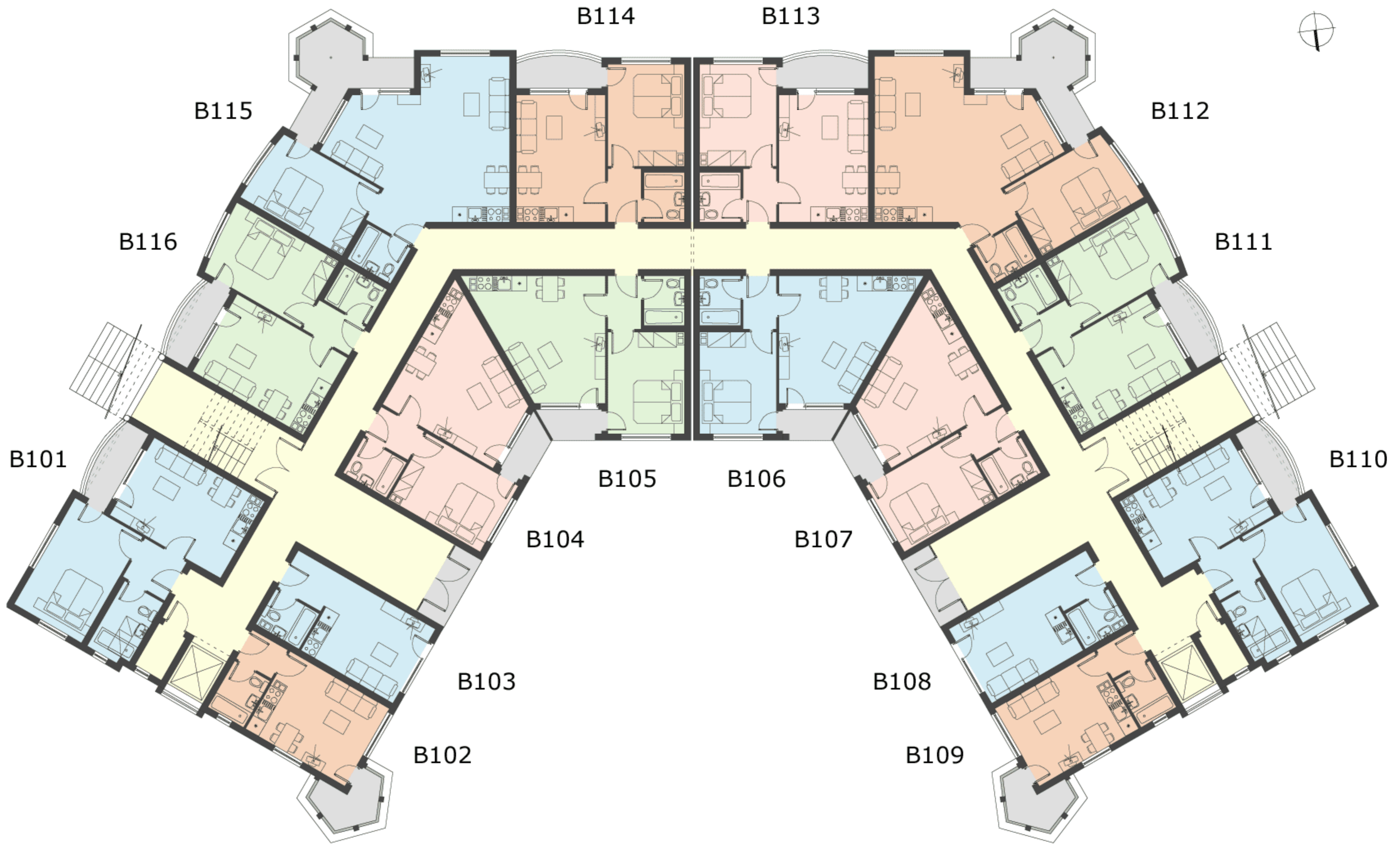
Block BI, floor 1 (±0.00)
